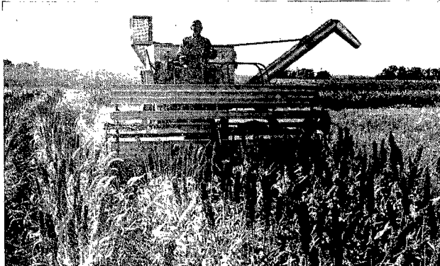
GLEANER combines have down-front cylinder, 2-fan cleaning, extra separating length, and quality construction. Save time and energy with big fuel and grain tanks, unloading on-the-go. Have new operator comfort with master group controls. Shown here — new Model E with 10-foot header, 12 feet of separating length, 40-bushel grain bin.
